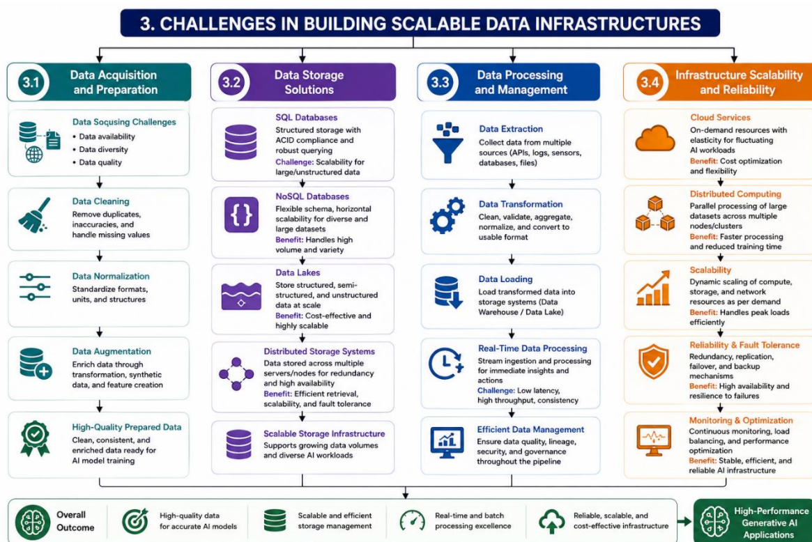
Fig 1 – Challenges in Building Scalable Data Infrastructures
