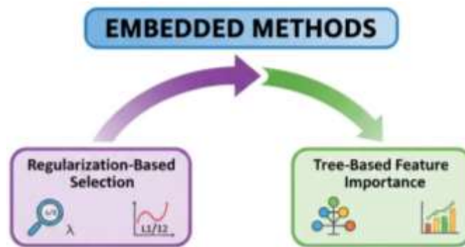
Fig 4 - Embedded Methods
