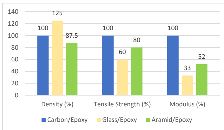
Fig 5 - Graph Representing Comparative Material Performance
